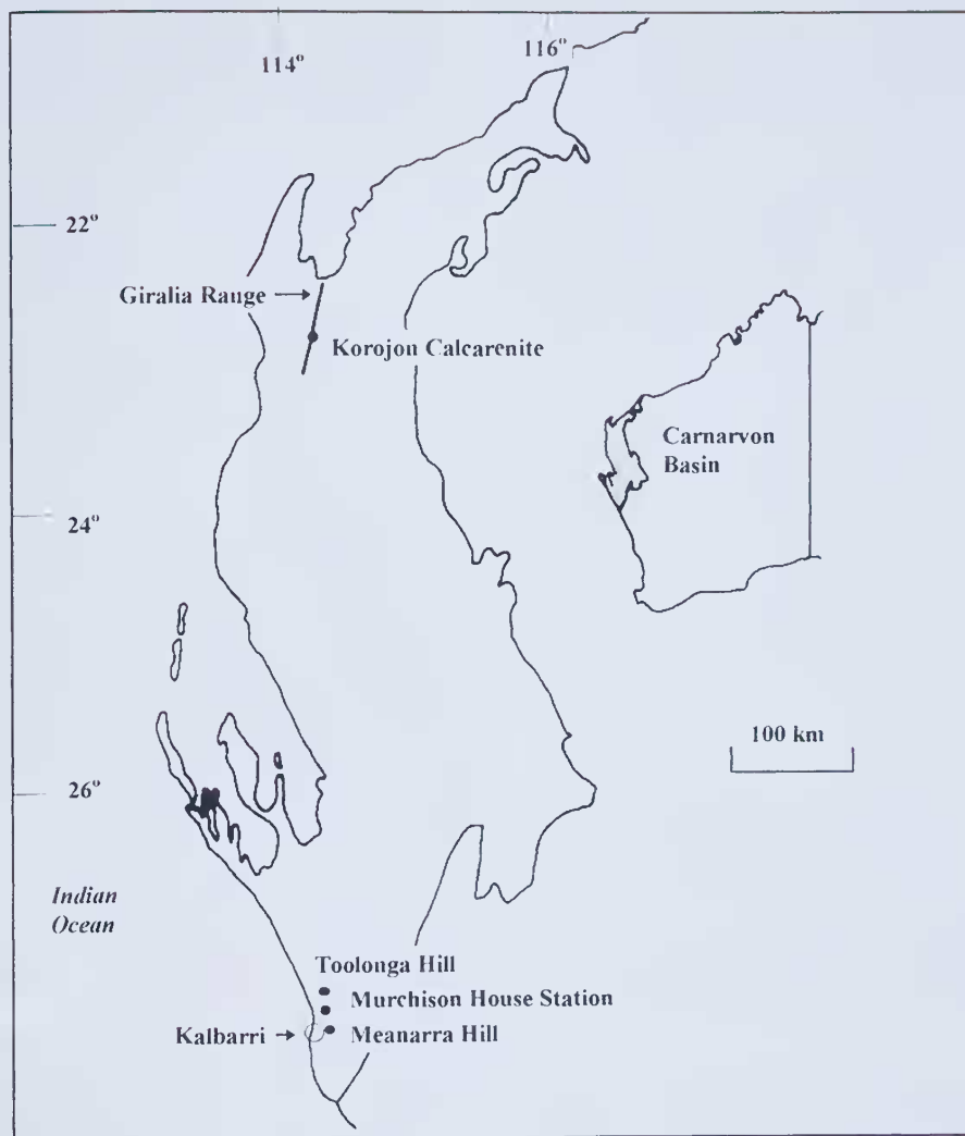
Figure 2 Late Cretaceous Toolonga Calcilutite (Toolonga Hill, Meanarra Hill and Murchison House Station) and Korojon Calcarenite (Giralia Range) in the Carnarvon Basin.
